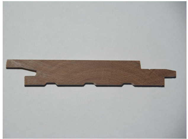
Allure Profile (secret fix, end matched): Standard Sizes 86x19 (65mm Cover) & 130x19 (110mm Cover)
